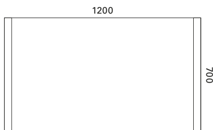
VIA VALOPEILI 120X70 • mitat L1200 x K700 x S60 mm
